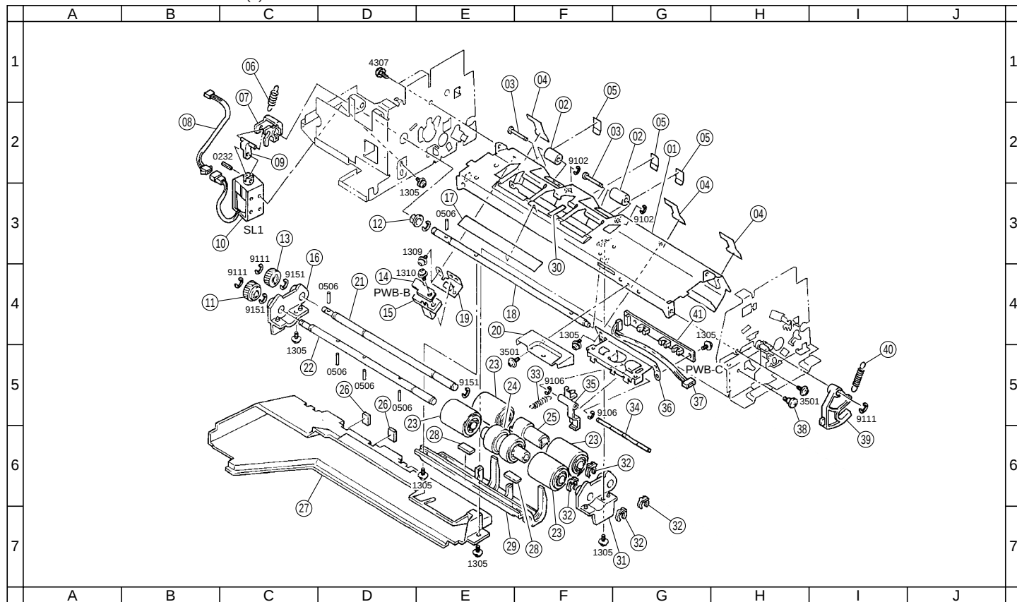
FIG. 3 PAPER TAKE-UP SECTION (II)
