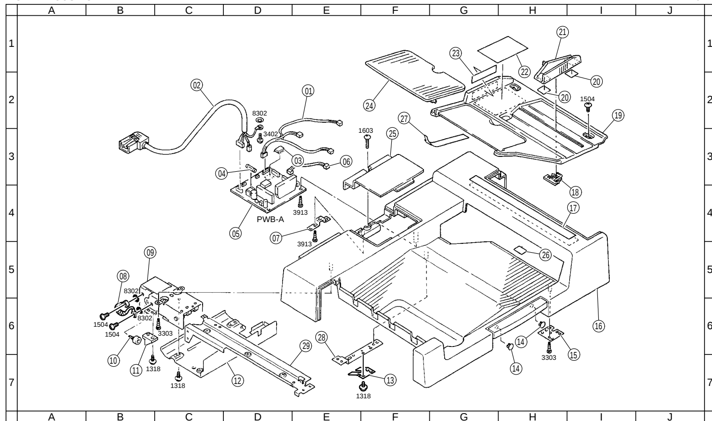
FIG. 1 HOUSING
