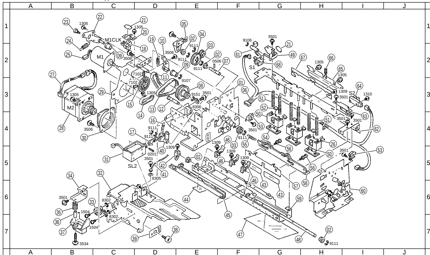
FIG. 2 PAPER TAKE-UP SECTION (I)
