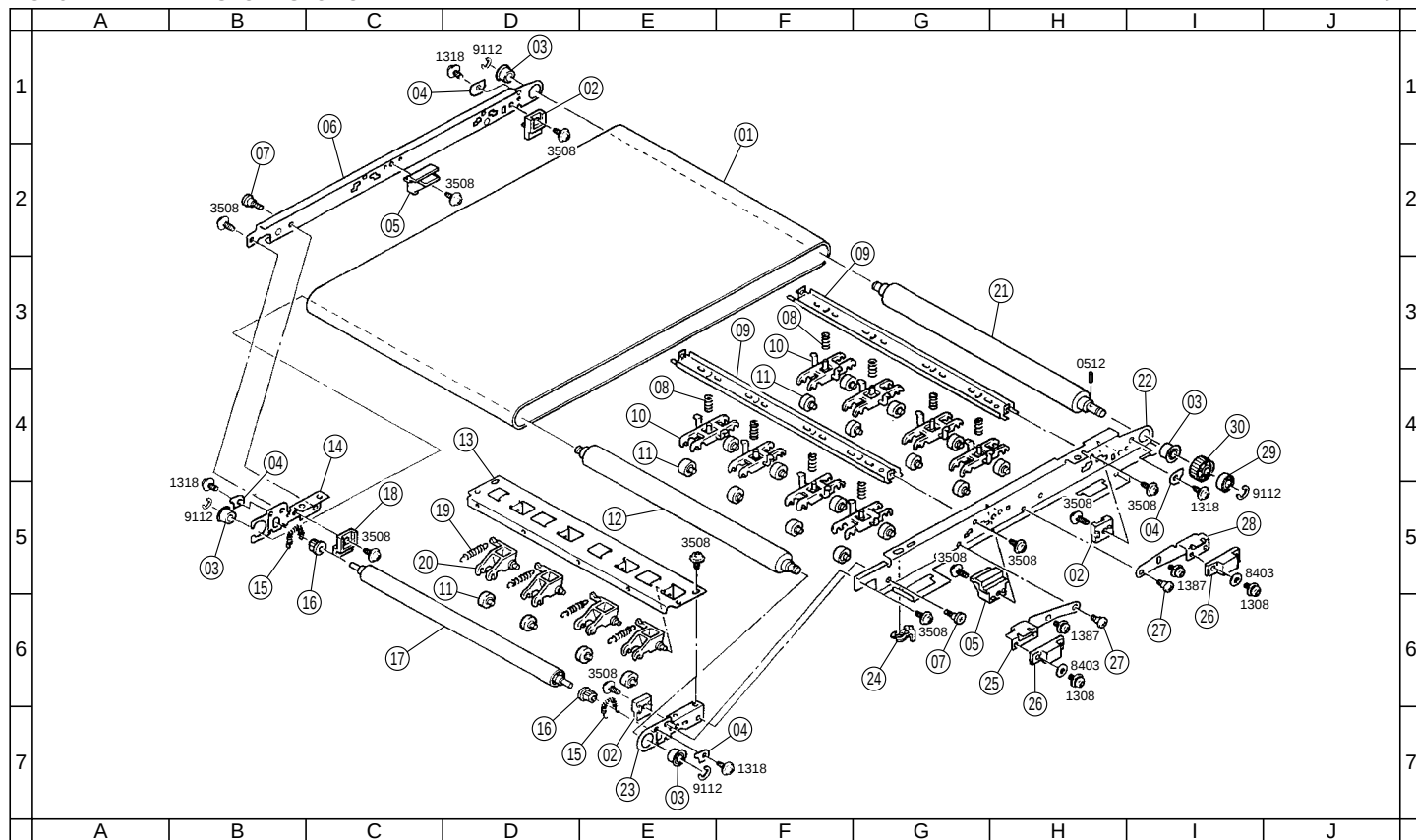
FIG. 5 PAPER TRANSPORT SECTION
