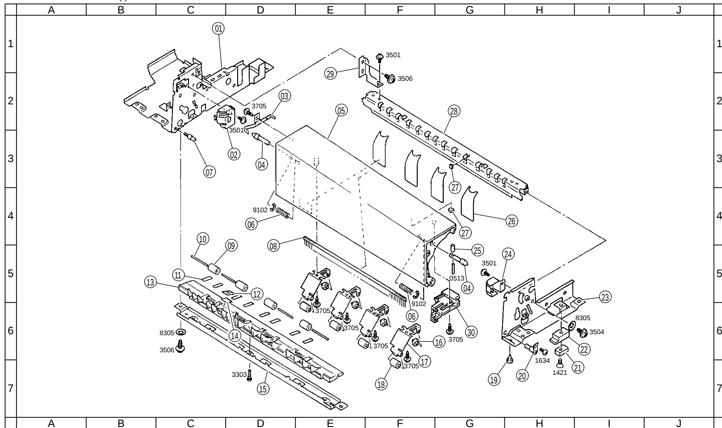
FIG. 6 EXIT SECTION (I)
